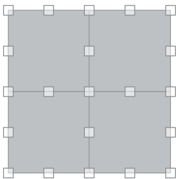
Quarter-Turn / Monolithic / Non-Directional (Random) Installation methods will require 3 TacTiles per square metre.
